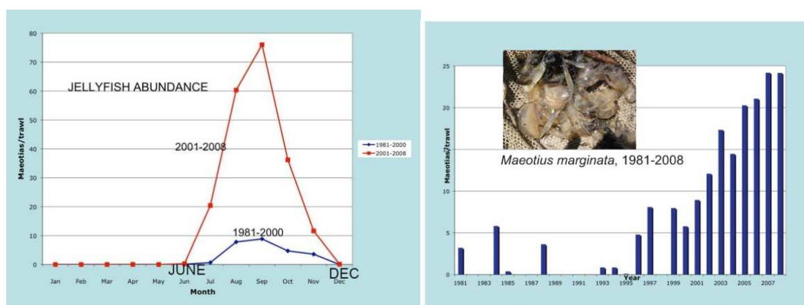
Figure 5.6.6. Invasive jellyfish abundance over time in Suisun Marsh (Moyle ppt. 2009).
