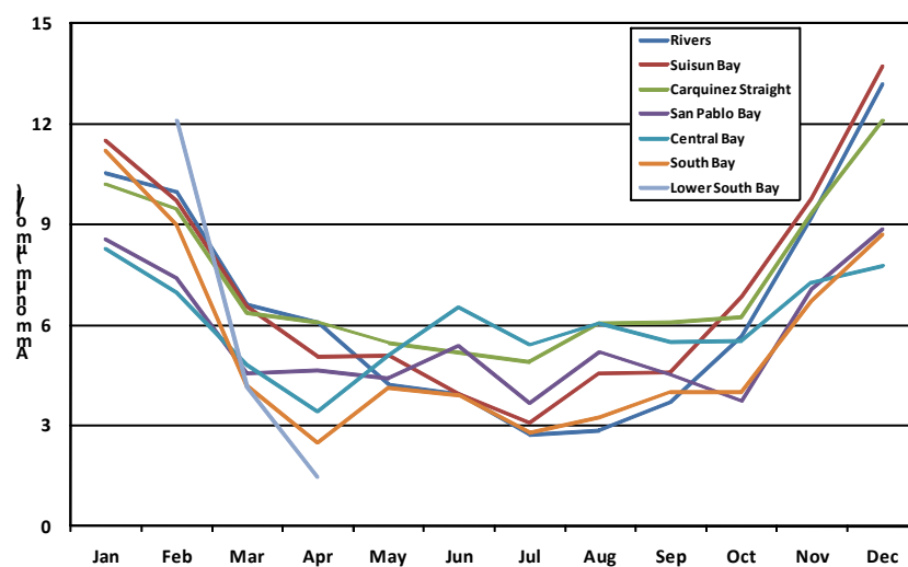
Figure 5.8.2. Monthly averaged ammonium concentrations in the defined segments of the San Francisco Bay for 1999 – 2010. Data obtained from the USGS: http://sfbay.wr.usgs.gov/access/wqdata ).
