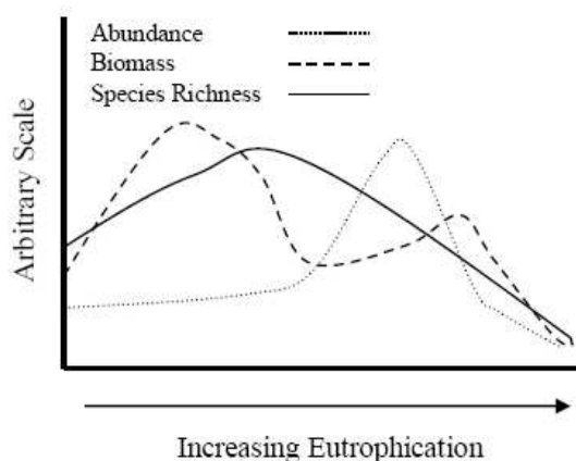
Figure 5.5.1. Conceptual patterns of abundance, biomass and species richness with increasing eutrophication. After Pearson and Rosenberg, 1978.
